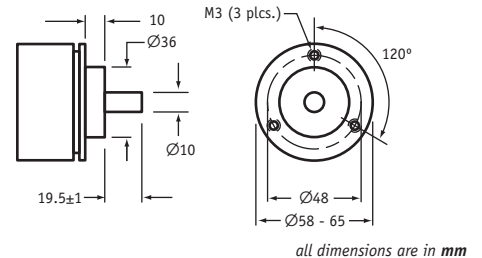
S04 - Face-Mount (10mm shaft/M3 screws)
